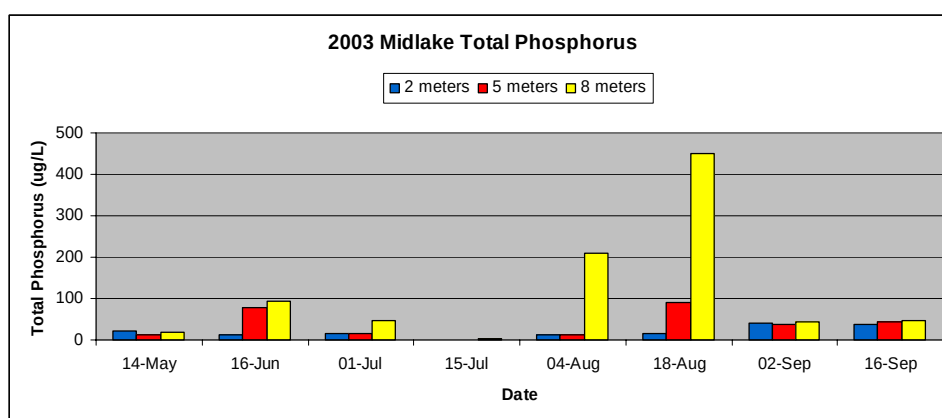
Figure 3-12: Phosphorus Levels 2003
