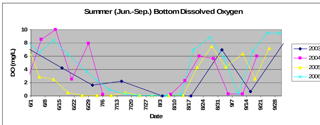
Figure 3-4: Bottom Dissolved Oxygen
