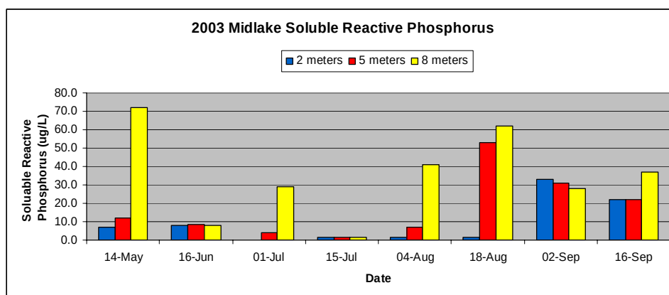
Figure 3-13: Soluble Reactive Phosphorus
