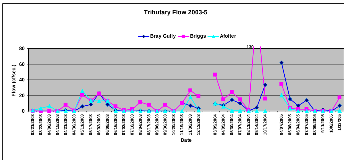
Figure 3-11: Tributary Flow 2003-2005
