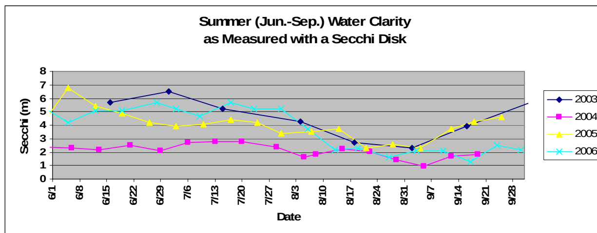
Figure 3-5: Water Clarity
